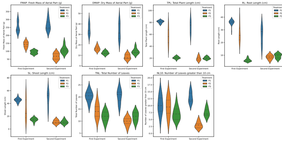
Figure 10: Agronomic measurements from the hydroponic deployment and comparison treatments. These data are included as secondary operation evidence for the closed-loop hydroponic platform. They are not interpreted as causal evidence that AASVR alone improved plant growth because multiple system-level factors differ between treatments.
