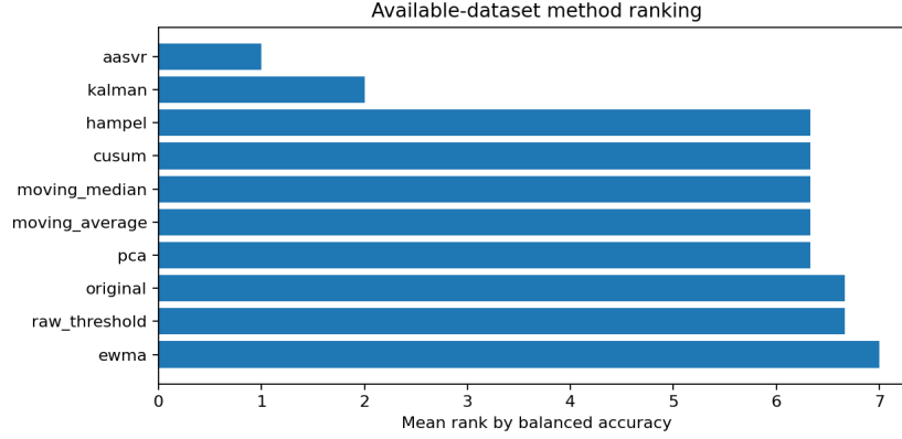
Figure 9: Mean rank by balanced accuracy across available benchmark tables. The ranking combines hydroponic synthetic faults with native-label external benchmark summaries. It is useful for orientation, but it should not be interpreted as a leaderboard because the datasets use different label semantics and evaluation units.
