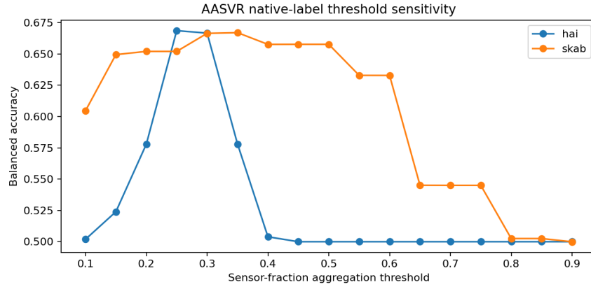
Figure 8: Threshold sensitivity for timestamp-level external labels. The fixed 30% aggregation rule is the headline protocol, but this plot shows how AASVR changes when the required fraction of rejecting streams is varied. SKAB is stable around the headline setting, while HAI reveals a tradeoff between recall and specificity.
